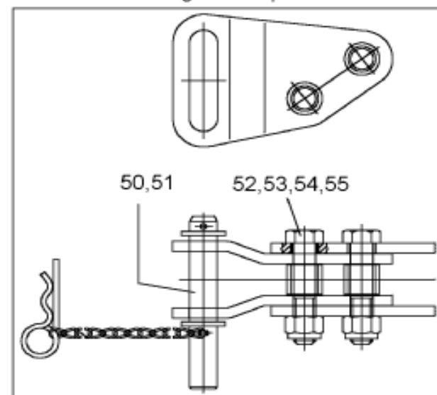
Langlochadapter
