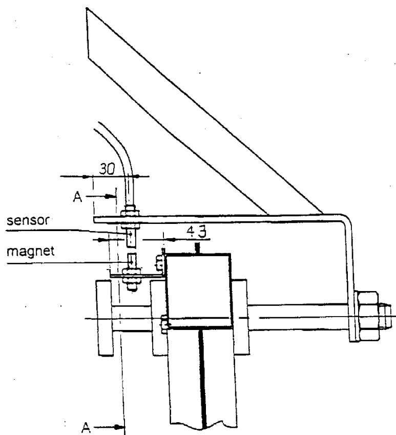
The mounting scheme for sensor of the working phas
