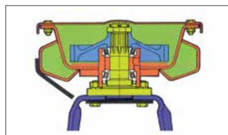
Lager unit HK 31 HY.
