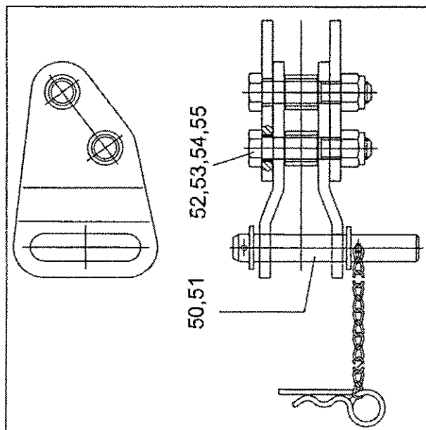
Langlochadapter
