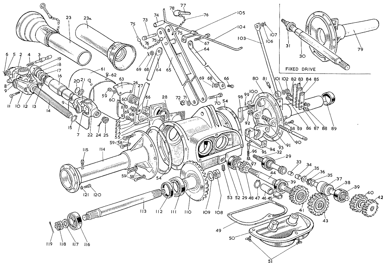
Diagram:- Universal Joint, Gearbox, R. H. Sideplate Jackshaft Assemblies
