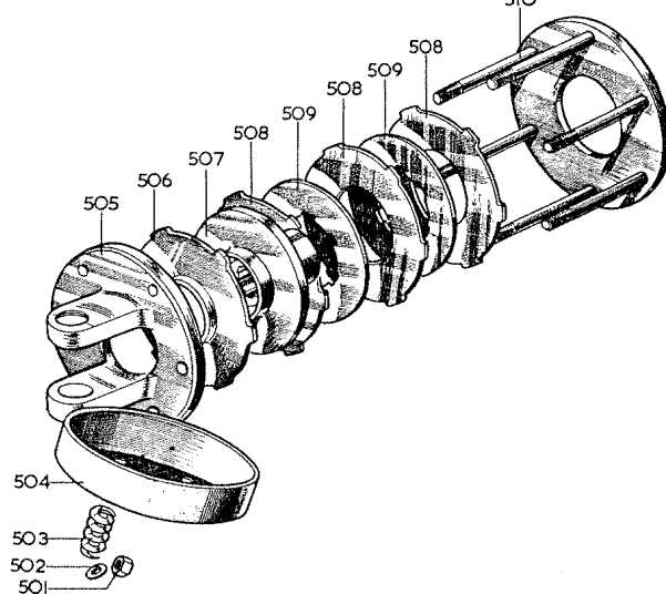
Diagram:- Clutch Assembly
