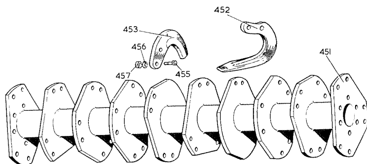
Diagram:- Picktime Rotor Assembly
