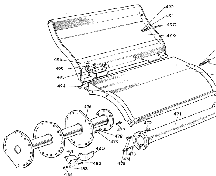
Diagram:- 30 Roto Extension Kit Assembly
