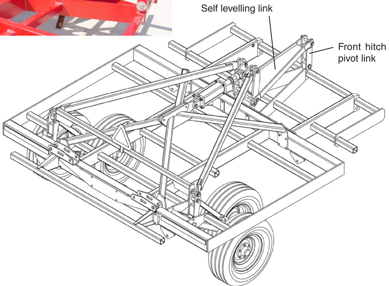
Overview of completed 10' (3m) self levelling linkage system.
