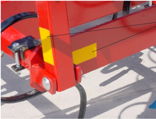
YELLOW REFLECTORS on both front corners and side bars of front frame.
