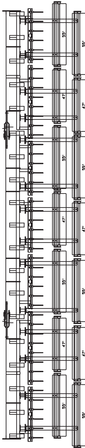
2800 CULTIVATOR 29'6" (9m) WIDTH - 4" (100mm) TINE SPACING (4m BASE) SPIKE BAR & DOUBLE SPIRAL HARROW LAYOUT SPIKE BAR - 603150548 DOUBLE ROLLER - 603150506
