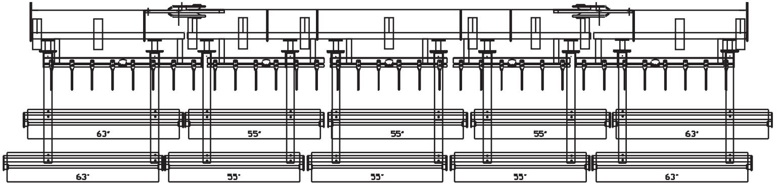
2800 CULTIVATOR 23'0" (7m) WIDTH - 6.25" (160mm) TINE SPACING (4m BASE) SPIKE BAR & DOUBLE SPIRAL HARROW LAYOUT SPIKE BAR - 603151007 DOUBLE ROLLER - 603151005
