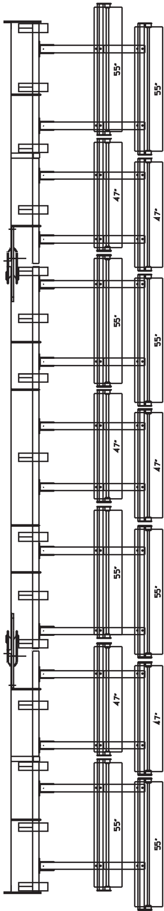
2800 CULTIVATOR 29'6" (9m) WIDTH - 6.25" (160mm) TINE SPACING (4m BASE) DOUBLE SPIRAL HARROW LAYOUT DOUBLE ROLLER - 603150506
