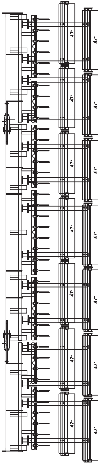
2800 CULTIVATOR 26'3" (8m) WIDTH - 6.25" (160mm) TINE SPACING (4m BASE) SPIKE BAR & DOUBLE SPIRAL HARROW LAYOUT SPIKE BAR - 603150547 DOUBLE ROLLER - 603150505
