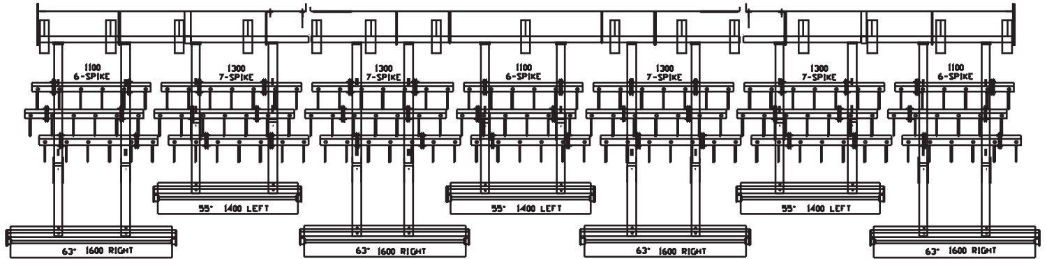
2800 CULTIVATOR 29'6" (9m) WIDTH - 6.25" (160mm) TINE SPACING (4m BASE) COMBI HARROW LAYOUT COMBI HARROW - 603150509
