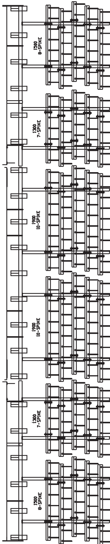
2800 CULTIVATOR 32'10" (10m) WIDTH - 4" (100mm) TINE SPACING (4m BASE) FLEX DRAG HARROW LAYOUT FLEX DRAG - 603150546
