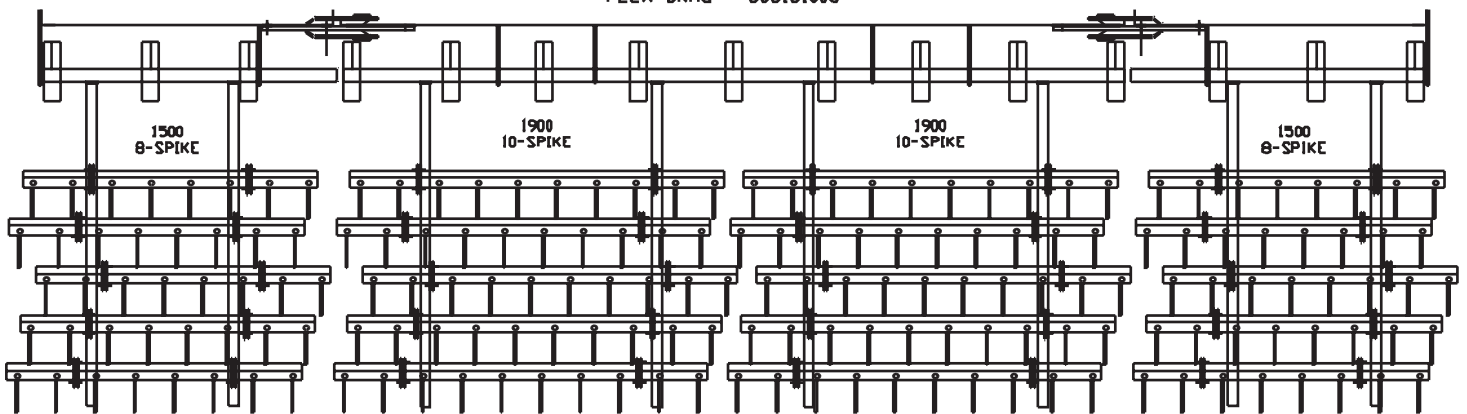
2800 CULTIVATOR 23'0" (7m) WIDTH - 4" (100mm) TINE SPACING (4m BASE) FLEX DRAG HARROW LAYOUT FLEX DRAG - 603151008
