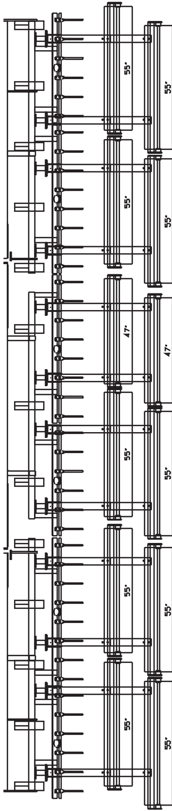
2800 CULTIVATOR 26'3" (8m) WIDTH - 6.25" (160mm) TINE SPACING (3m BASE) SPIKE BAR & DOUBLE SPIRAL HARROW LAYOUT SPIKE BAR - 603150103 DOUBLE ROLLER - 603150095
