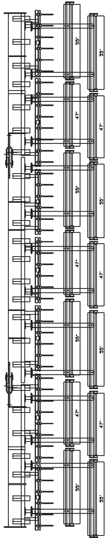
2800 CULTIVATOR 29'6" (9m) WIDTH - 3" (80mm) TINE SPACING (4m BASE) SPIKE BAR & DOUBLE SPIRAL HARROW LAYOUT SPIKE BAR - 603150548 DOUBLE ROLLER - 603150506
