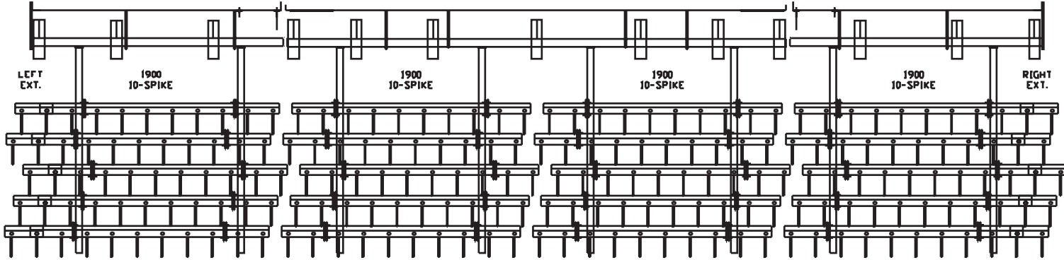
2800 CULTIVATOR 26'3" (8m) WIDTH - 6.25" (160mm) TINE SPACING (4m BASE) FLEX DRAG HARROW LAYOUT FLEX DRAG - 603150544
