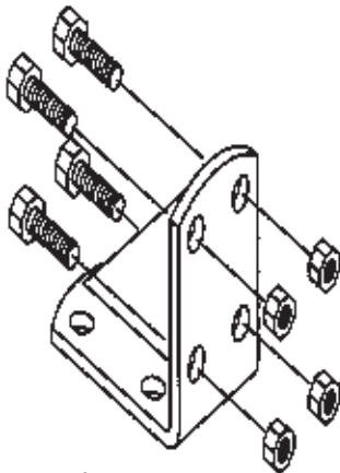
603150995 COMBI & DRAG HARROW HEIGHT BRACKET ASSEMBLY FOR 2800 & 3800 WITH 20" CONSER-TINES
