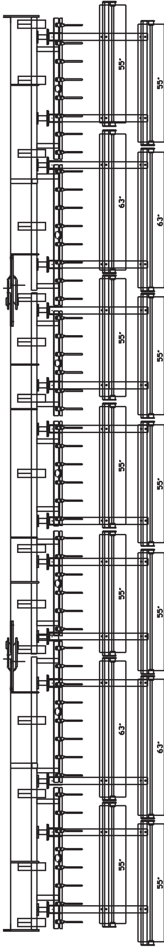
2800 CULTIVATOR 32'10" (10m) WIDTH - 6.25" (160mm) TINE SPACING (4m BASE) SPIKE BAR & DOUBLE SPIRAL HARROW LAYOUT SPIKE BAR - 603150549 DOUBLE ROLLER - 603150507
