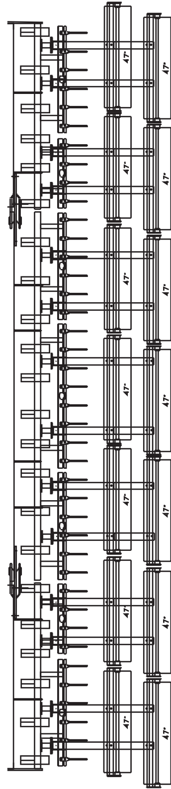
2800 CULTIVATOR 26'3" (8m) WIDTH - 3" (80mm) TINE SPACING (4m BASE) SPIKE BAR & DOUBLE SPIRAL HARROW LAYOUT SPIKE BAR - 603150547 DOUBLE ROLLER - 603150505
