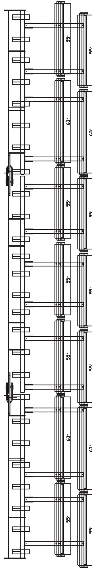
2800 CULTIVATOR 32'10" (10m) WIDTH - 3" (80mm) TINE SPACING (4m BASE) DOUBLE SPIRAL HARROW LAYOUT DOUBLE ROLLER - 603150507
