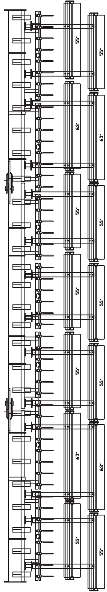
2800 CULTIVATOR 32'10" (10m) WIDTH - 3" (80mm) TINE SPACING (4m BASE) SPIKE BAR & DOUBLE SPIRAL HARROW LAYOUT SPIKE BAR - 603150549 DOUBLE ROLLER - 603150507
