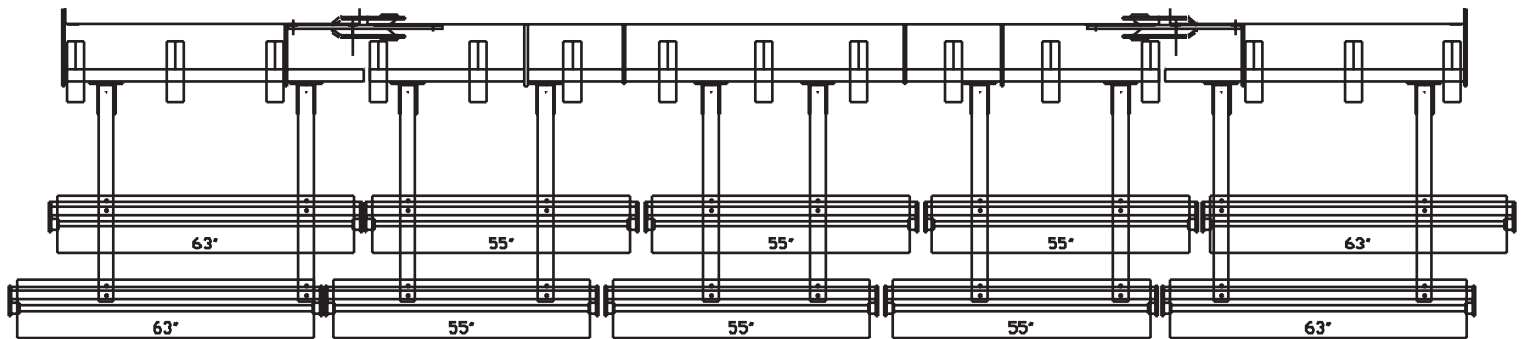
2800 CULTIVATOR 23'0" (7m) WIDTH - 4" (100mm) TINE SPACING (4m BASE) DOUBLE SPIRAL HARROW LAYOUT DOUBLE ROLLER - 603151005
