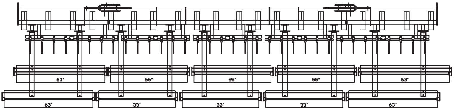
2800 CULTIVATOR 23'0" (7m) WIDTH - 3" (80mm) TINE SPACING (4m BASE) SPIKE BAR & DOUBLE SPIRAL HARROW LAYOUT SPIKE BAR - 603151007 DOUBLE ROLLER - 603151005
