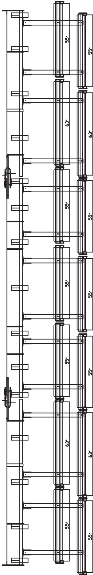
2800 CULTIVATOR 32'10" (10m) WIDTH - 6.25" (160mm) TINE SPACING (4m BASE) DOUBLE SPIRAL HARROW LAYOUT DOUBLE ROLLER - 603150507
