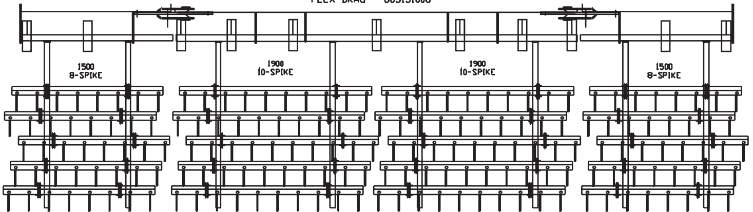
2800 CULTIVATOR 23'0" (7m) WIDTH - 6.25" (160mm) TINE SPACING (4m BASE) FLEX DRAG HARROW LAYOUT FLEX DRAG - 603151008
