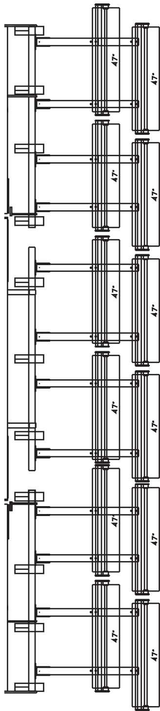
2800 CULTIVATOR 23'0" (7m) WIDTH - 6.25" (160mm) TINE SPACING (3m BASE) DOUBLE SPIRAL HARROW LAYOUT DOUBLE ROLLER - 603150484
