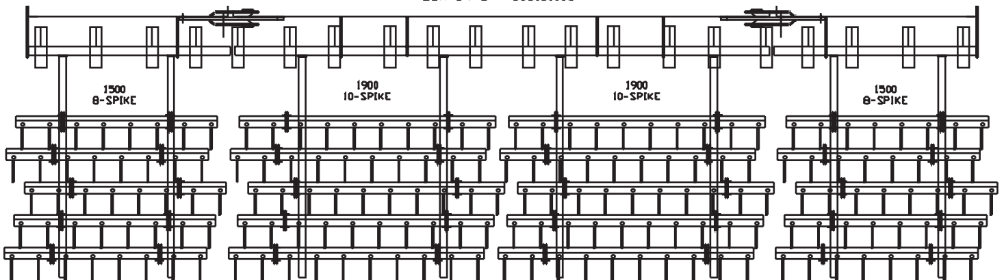
2800 CULTIVATOR 23'0" (7m) WIDTH - 3" (80mm) TINE SPACING (4m BASE) FLEX DRAG HARROW LAYOUT FLEX DRAG - 603151008
