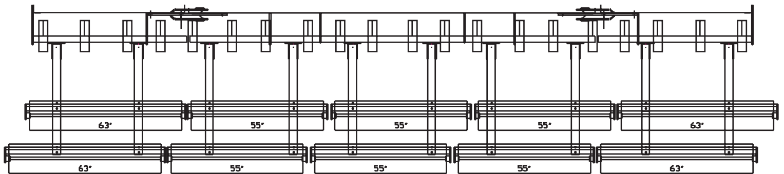
2800 CULTIVATOR 23'0" (7m) WIDTH - 3" (80mm) TINE SPACING (4m BASE) DOUBLE SPIRAL HARROW LAYOUT DOUBLE ROLLER - 603151005
