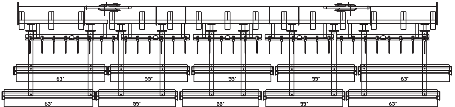
2800 CULTIVATOR 23'0" (7m) WIDTH - 4" (100mm) TINE SPACING (4m BASE) SPIKE BAR & DOUBLE SPIRAL HARROW LAYOUT SPIKE BAR - 603151007 DOUBLE ROLLER - 603151005
