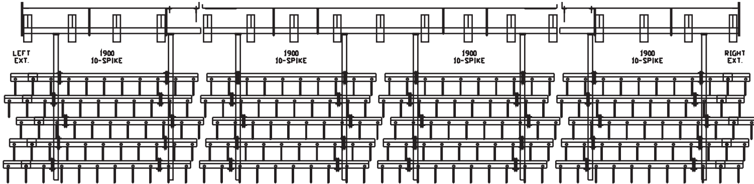
2800 CULTIVATOR 26'3" (8m) WIDTH - 4" (100mm) TINE SPACING (4m BASE) FLEX DRAG HARROW LAYOUT FLEX DRAG - 603150544
