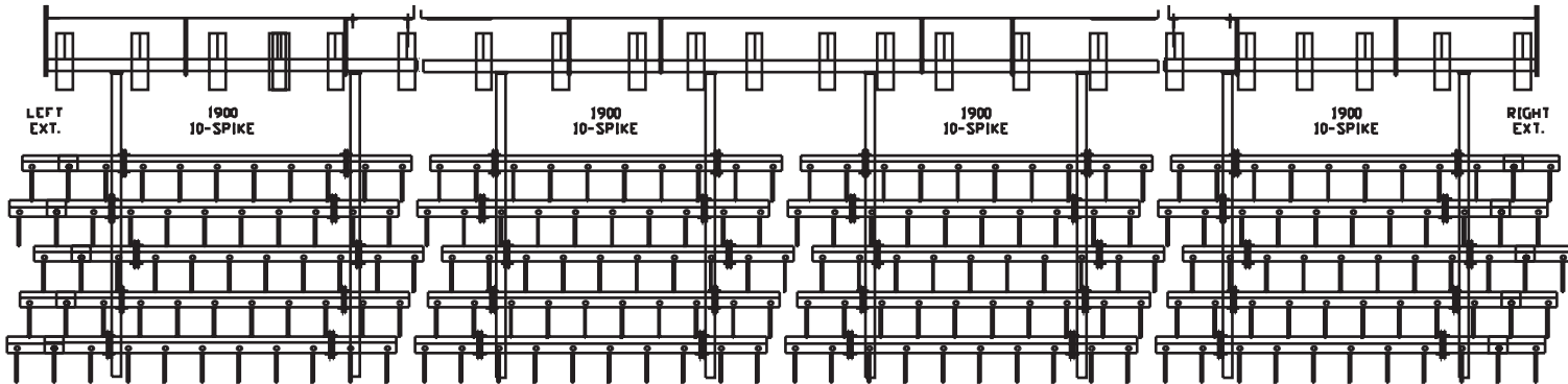
2800 CULTIVATOR 26'3" (8m) WIDTH - 3" (80mm) TINE SPACING (4m BASE) FLEX DRAG HARROW LAYOUT FLEX DRAG - 603150544
