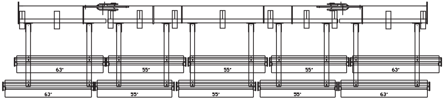
2800 CULTIVATOR 23'0" (7m) WIDTH - 6.25" (160mm) TINE SPACING (4m BASE) DOUBLE SPIRAL HARROW LAYOUT DOUBLE ROLLER - 603151005
