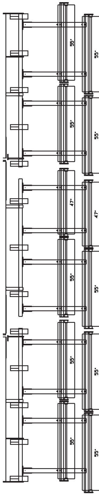
2800 CULTIVATOR 26'3" (8m) WIDTH - 6.25" (160mm) TINE SPACING (3m BASE) DOUBLE SPIRAL HARROW LAYOUT DOUBLE ROLLER - 603150095
