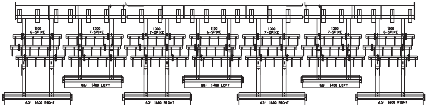
2800 CULTIVATOR 29'6" (9m) WIDTH - 3" (80mm) TINE SPACING (4m BASE) COMBI HARROW LAYOUT COMBI HARROW - 603150509
