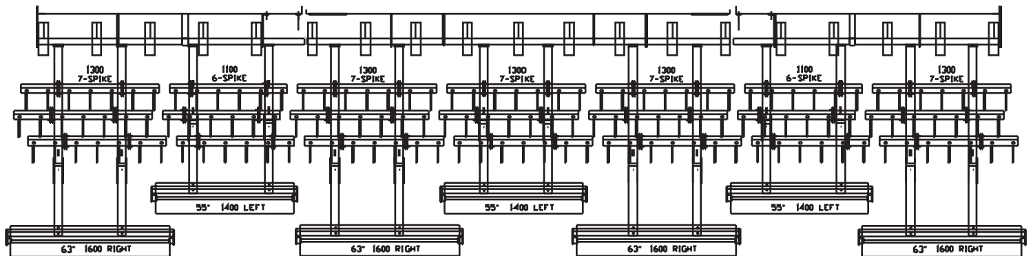
2800 CULTIVATOR 29'6" (9m) WIDTH - 4" (100mm) TINE SPACING (4m BASE) COMBI HARROW LAYOUT COMBI HARROW - 603150509
