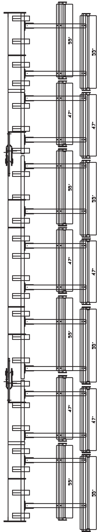
2800 CULTIVATOR 29'6" (9m) WIDTH - 3" (80mm) TINE SPACING (4m BASE) DOUBLE SPIRAL HARROW LAYOUT DOUBLE ROLLER - 603150506
