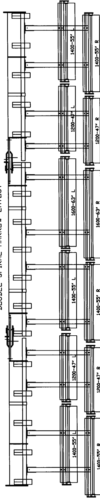
2800 CULTIVATOR 26'3" (8M) WIDTH - 4' (100MM) TINE SPACING DOUBLE SPIRAL HARROW LAYOUT
