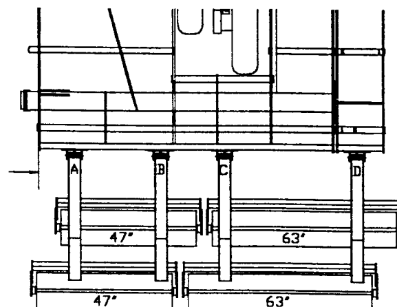
31' WINGS ROLLER SIZE LOCATIONS
