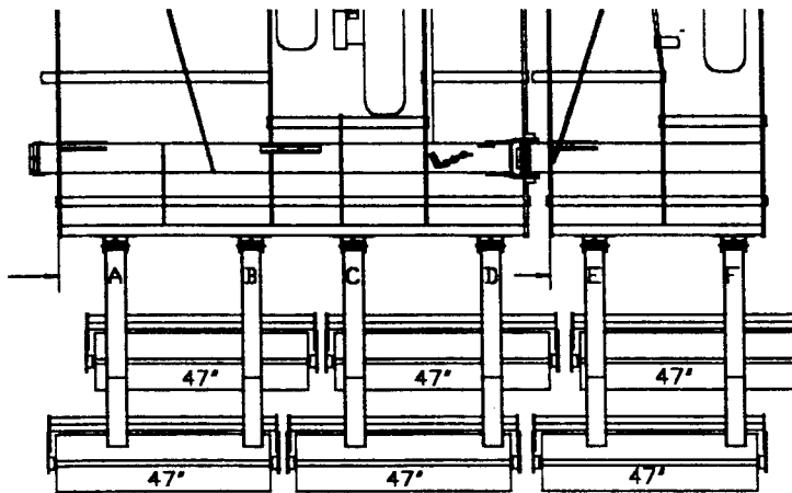
36' WINGS ROLLER SIZE LOCATIONS
