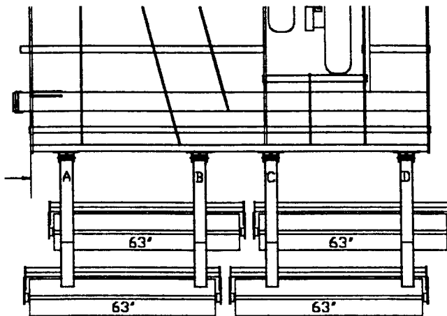
34' WINGS ROLLER SIZE LOCATIONS
