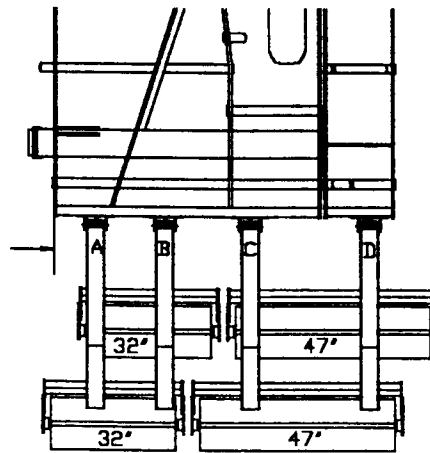
25' WINGS ROLLER SIZE LOCATIONS
