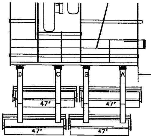
28' WINGS ROLLER SIZE LOCATIONS
