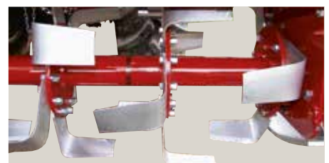
Detail of the bladed rotor.
